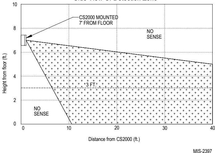
Side View Of Detection Zone
