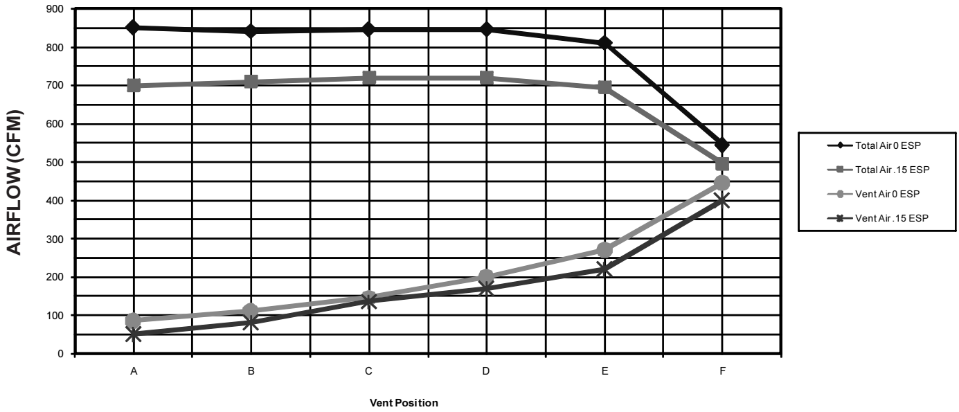
S26H1 & S31H1 High Speed Total and Ventilation Airflow
