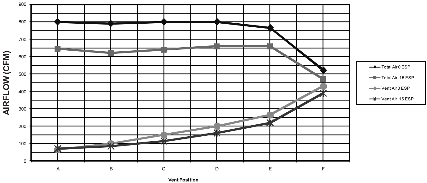
S26H1 & S31H1 Low Speed Total and Ventilation Airflow
